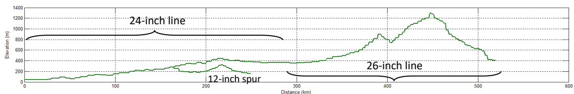
Figure 3 – Elevation of the 24-inch and the 26-inch lines and the 12-inch spur line. The line elevation is an input into the model.
