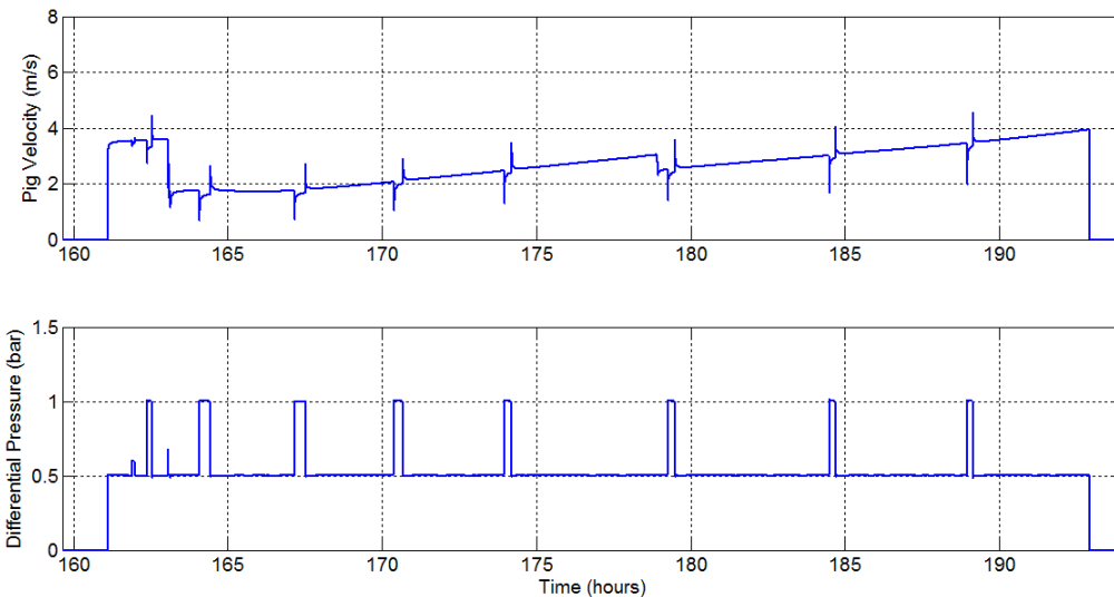
Figure 17 – Reduced flow for 24 hours while the system adjusts to allow pigging to take place. Note the time taken for flow to recover. This is due to the compressibility of the gas.
