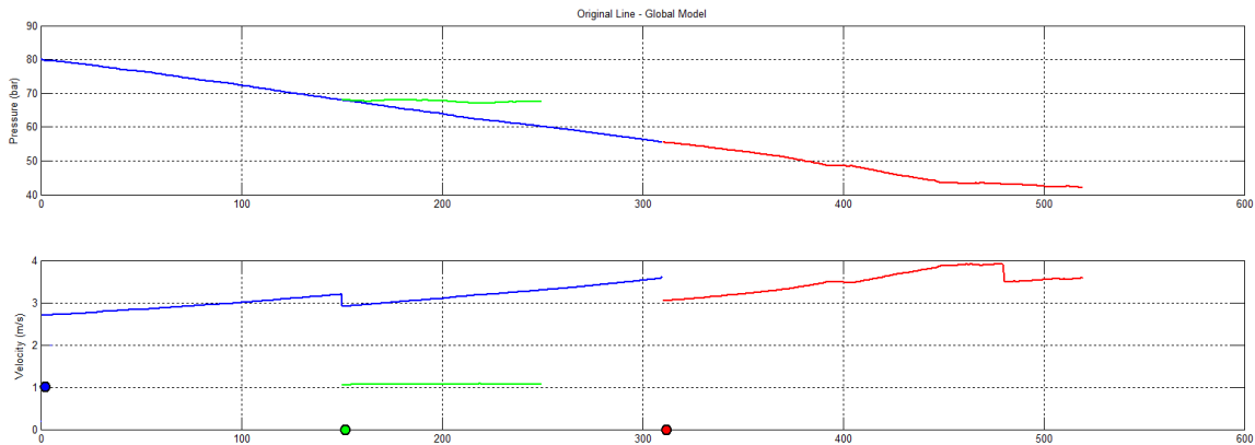
Figure 6 – Steady state pressure and flow velocity in the line along the length of the three pipelines (24-inch in blue, 26-inch in red and 12-inch in green). The pigs, in corresponding blue, red and green are shown ready to launch.
