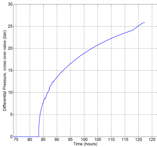
Figure 27 – Pressure drop across the various valve in the system during the last pigging operation. An excessive pressure drop is noted across the cross over valve making this method of pigging untenable.
