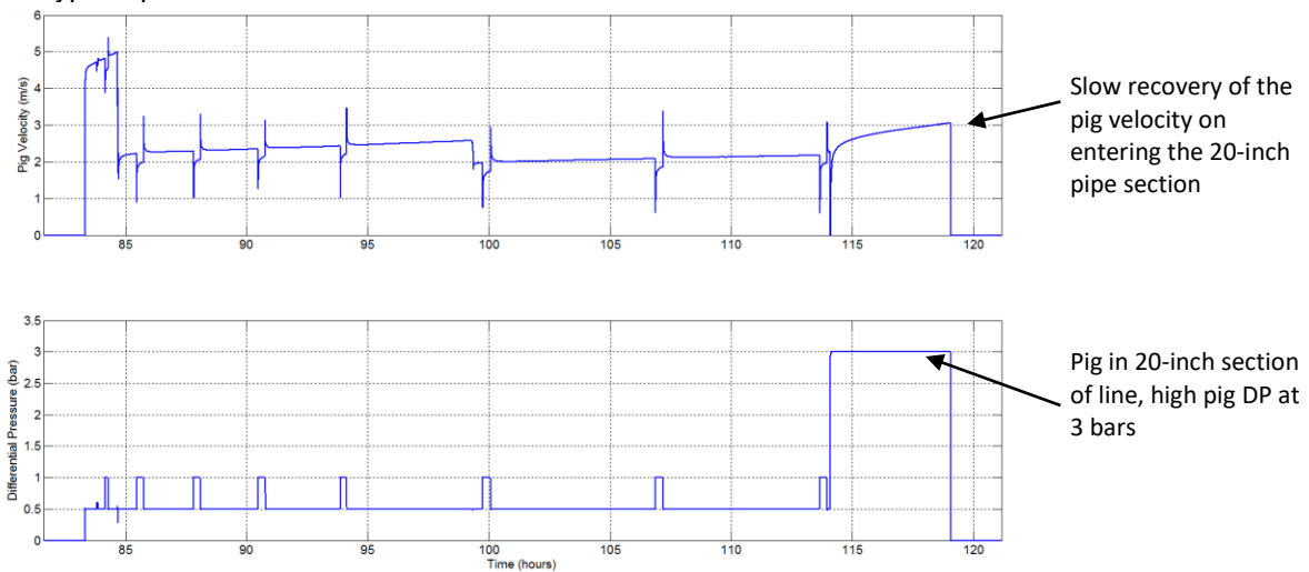
Figure 23 - Pig velocity against time with pig differential pressure shown. The pig initially stalls as it enters the 20-inch section of the line. There is then a very slow recovery of pig velocity. This is due to diversion of flow into the parallel line.
